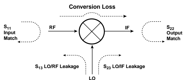
Diagram showing typical mixer measurements easily tested using Scorpion.
