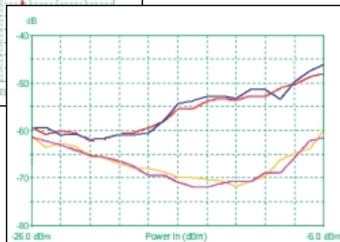
ACPR Versus Power
