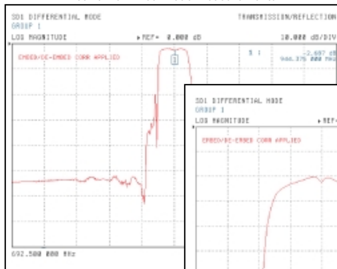
Real-time Mixed-Mode Measurements
